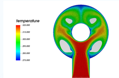
圆盘注塑
